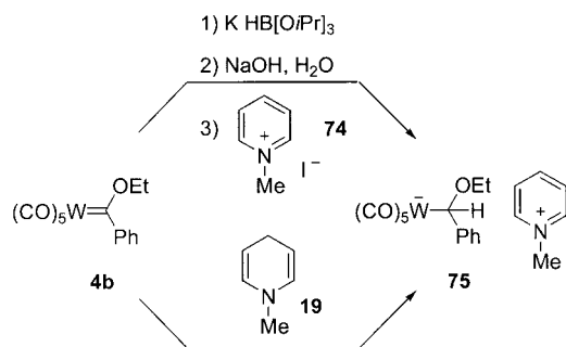
Scheme 29
