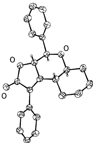
Figure 1. X-ray structure of the butenolide 53k (CAMERON view), atoms drawn at 50% probability
