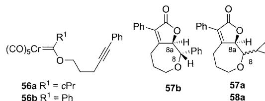
Scheme 22
