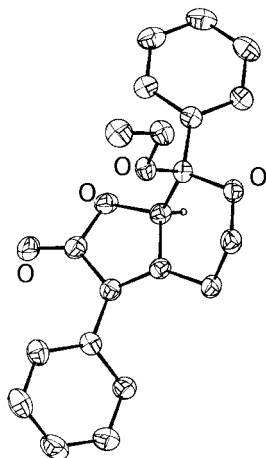
Figure 3. X-ray structure of the butenolide 84 (CAMERON view), atoms are drawn at 50% probability
