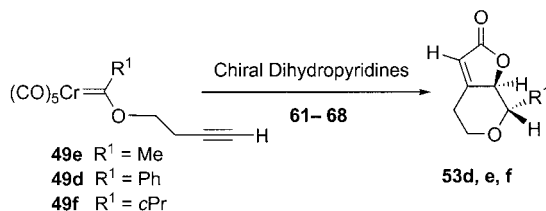
Scheme 25
