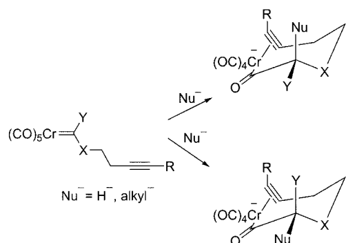
Scheme 42
