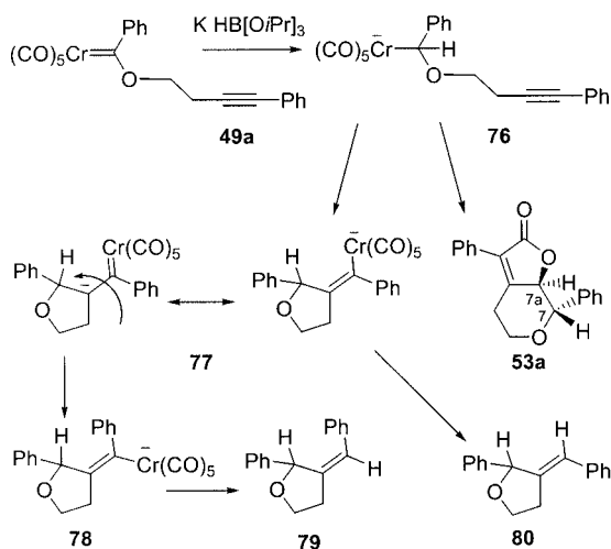
Scheme 30
