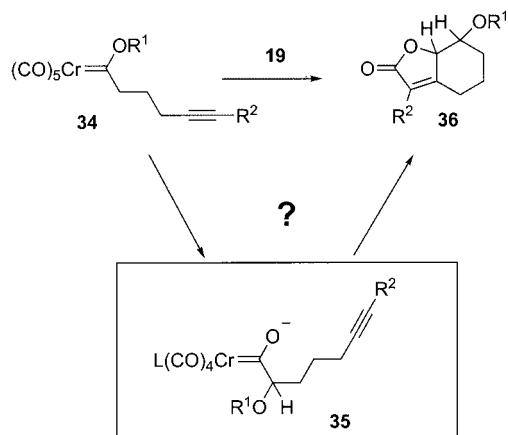
Scheme 10
