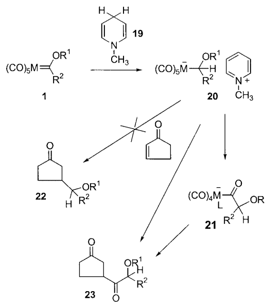
Scheme 6
