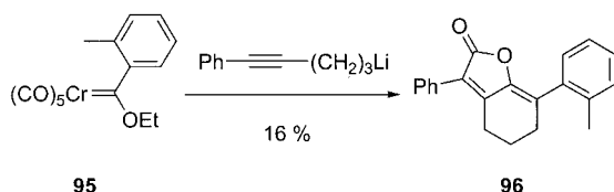
Scheme 38
