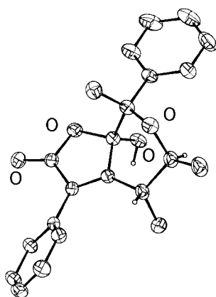
Figure 4. X-ray structure of the butenolide 91 (CAMERON view), atoms are drawn at 50% probability
