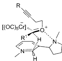
Figure 5. Transition-state model for the interaction of N -methyldihydronicotine with a carbene complex
