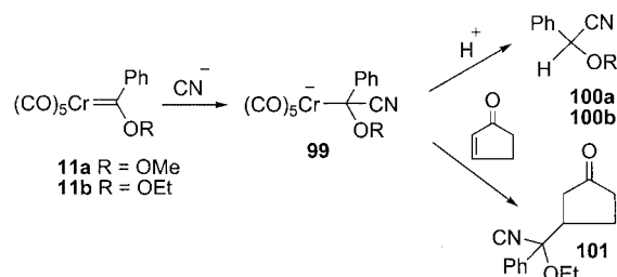
Scheme 40
