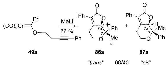
Scheme 33
