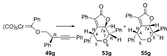
Scheme 20
