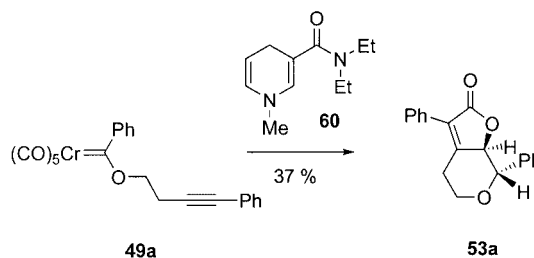
Scheme 24
