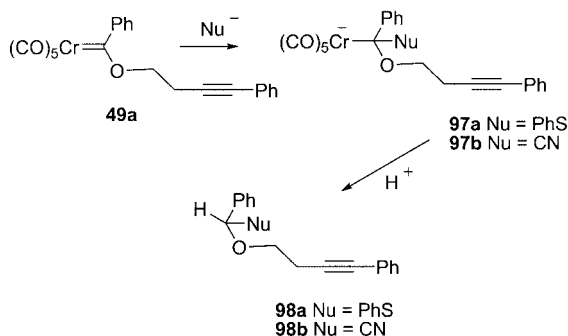
Scheme 39
