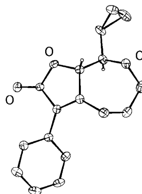
Figure 2. X-ray structure of the butenolide 57a (CAMERON view), atoms drawn at 50% probability
