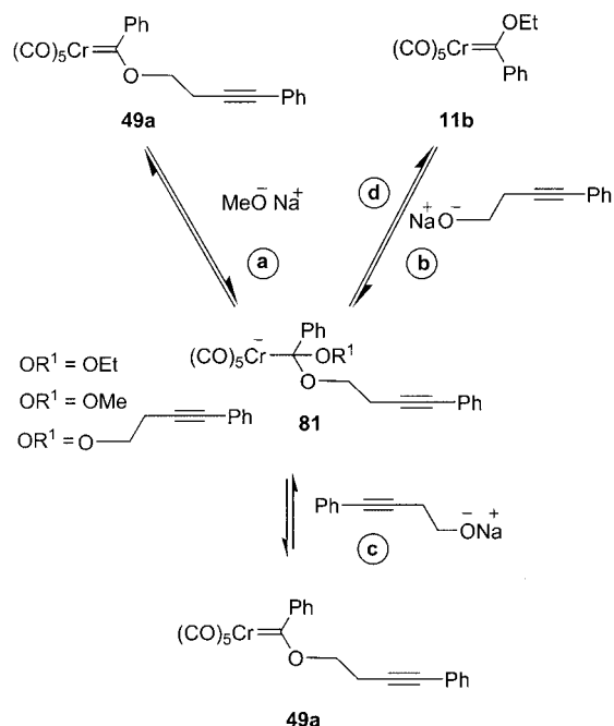
Scheme 31
