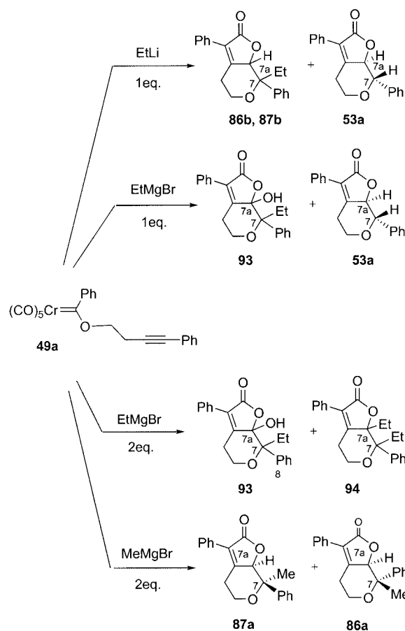
Scheme 37
