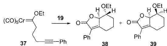
Scheme 11
