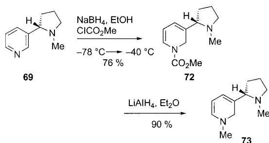
Scheme 27
